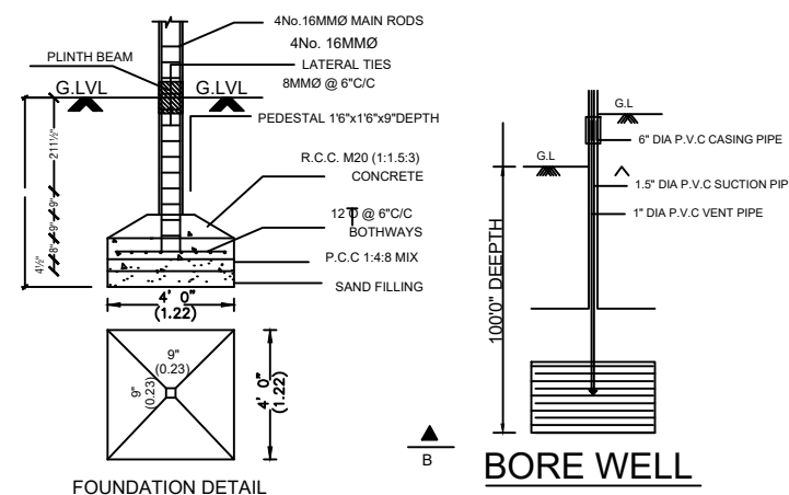
FOUNDATION DETAIL
