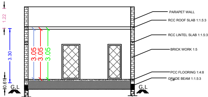
SECTION AT A,B
