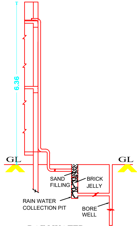
RAIN WATER HARVESTING SYSTEM
