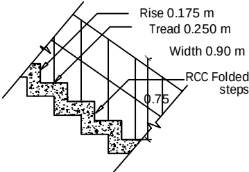
STAIRCASE DETAILS
