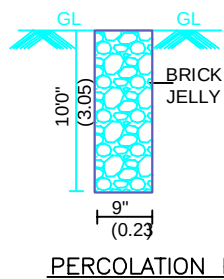
PERCOLATION PIT
