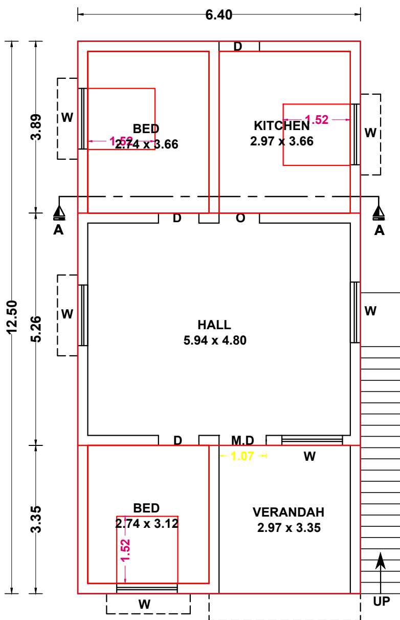
EXI. & PRO. GROUND FLOOR PLAN
