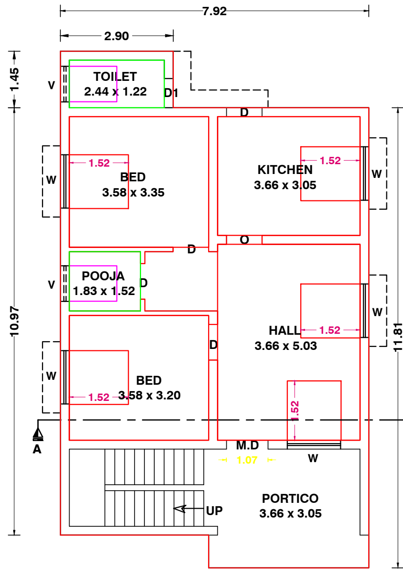
PLAN
