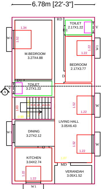
PRO.GROUND FLOOR PLAN
