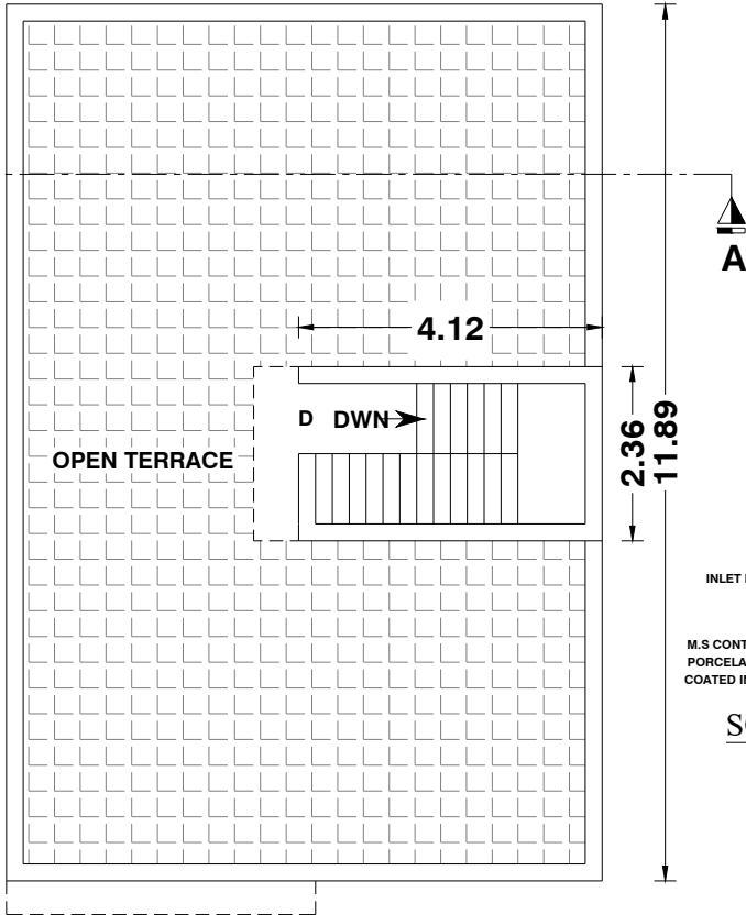
TERRACE FLOOR PLAN NON FSI
