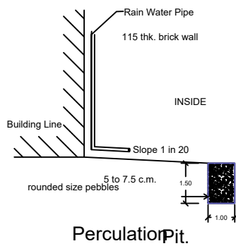
RAINWATER HARVESTING
