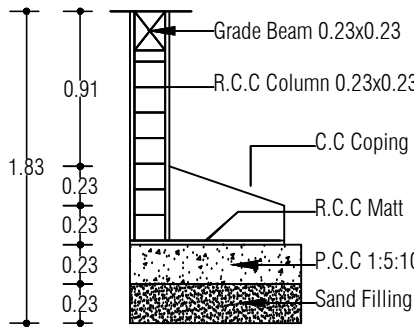
Foundation Details
