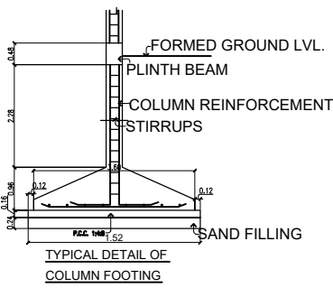
TYPICAL DETAIL OF COLUMN FOOTING
