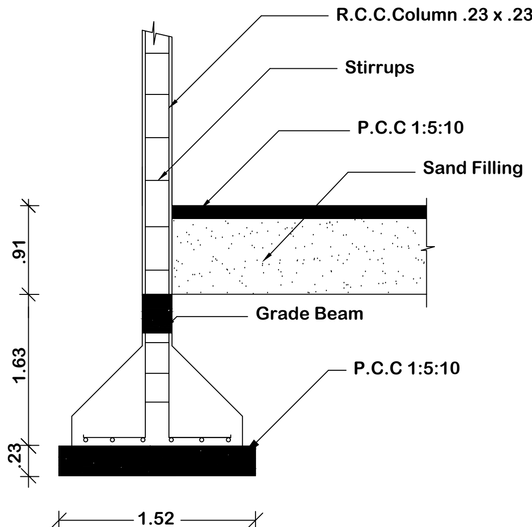
COLUMN DETAIL
