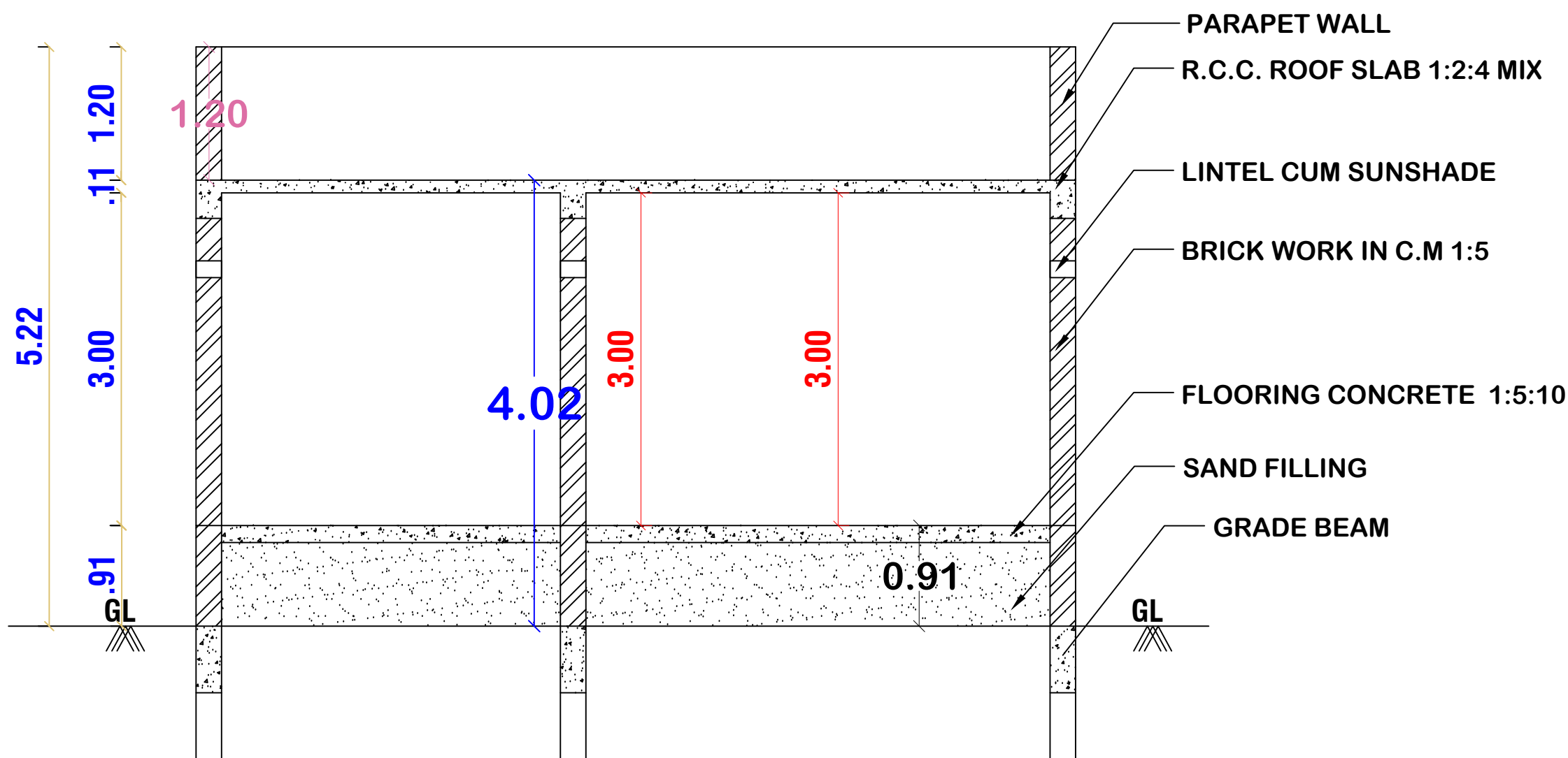
SECTION-"AA"
