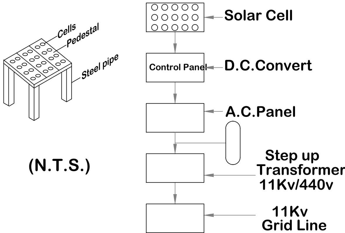
SOLAR SYSTEM FLOW DIAGRAM
