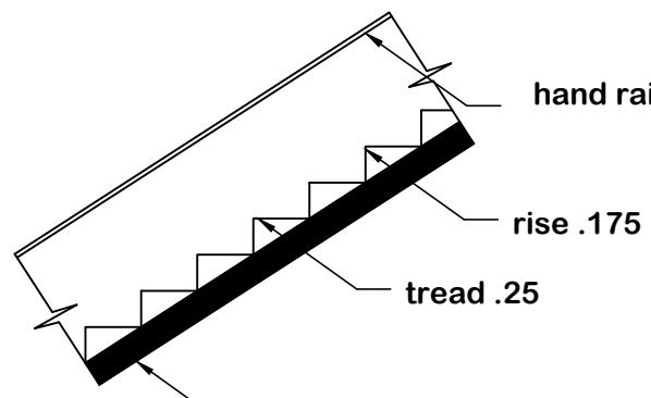
STAIR
