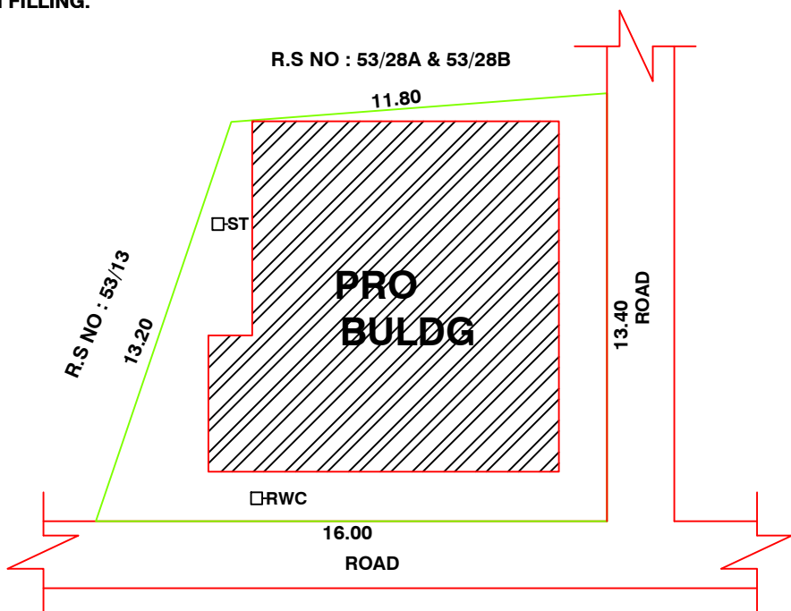
SITE PLAN (NOT TO SCALE)
