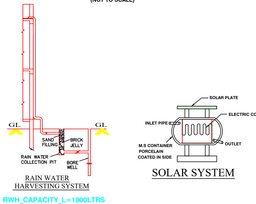
RAIN WATER HARVESTING SYSTEM RWH_CAPACITY_L=1000LTRS
