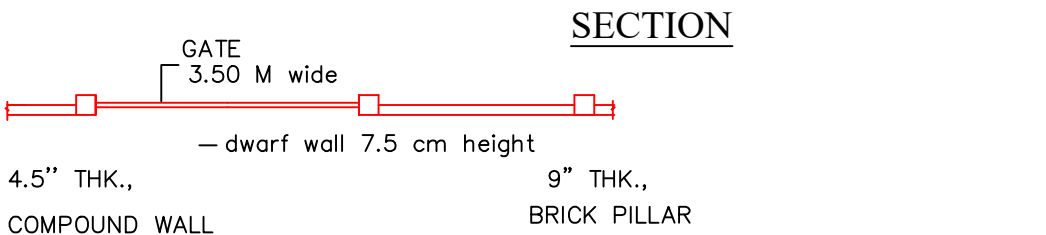
COMPOUND WALL PLAN
