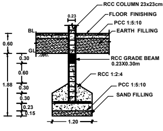
FOUNDATION DETAILS
