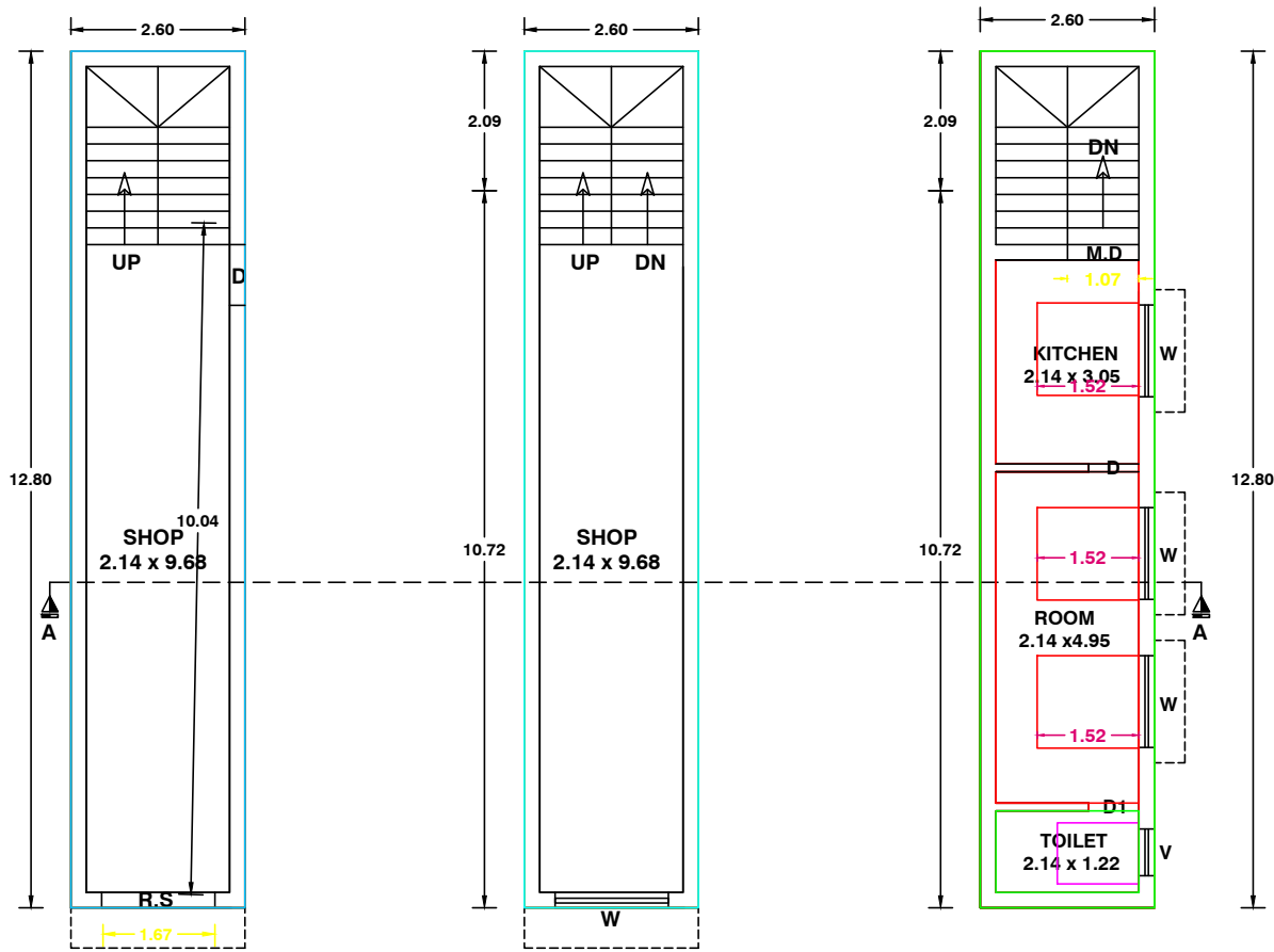
EXI.&REV.GROUND FLOOR PLAN
