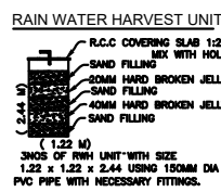
RAIN WATER HARVEST UNIT
