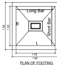
PLAN OF FOOTING
