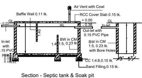
Section - Septic tank & Soak pit
