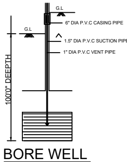
BORE WELL
