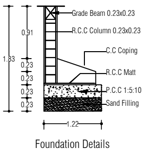
Foundation Details
