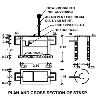
PLAN AND CROSS SECTION OF ST&SP.
