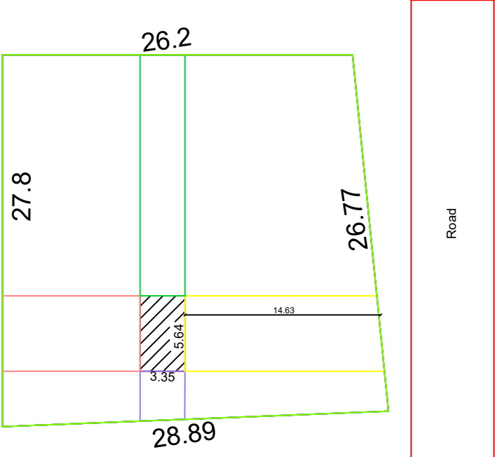
Site Plan
