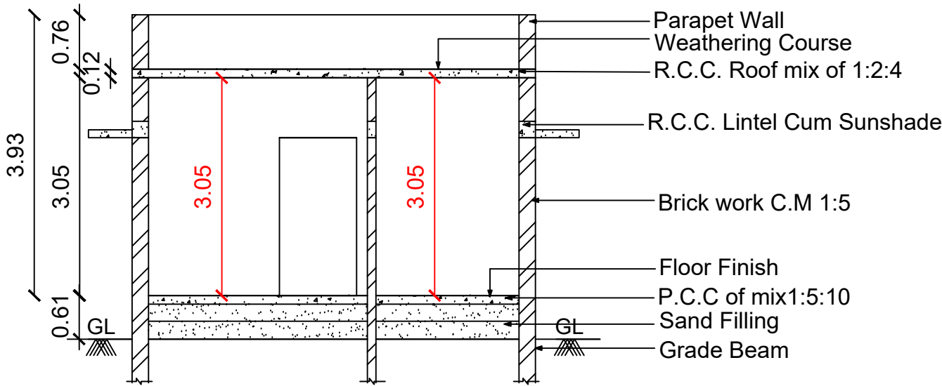
CROSS SECTION AB
