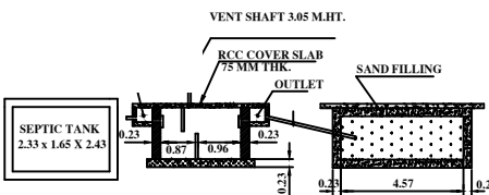
PLAN & SECTION ON SEPTIC TANK & DISP-TRENCH
