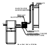
RAIN WATER HARVESTING SYSTEM
