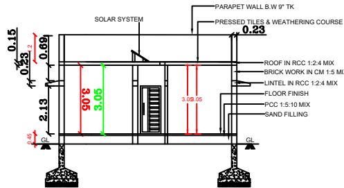
CROSS SECTION AB
