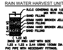
RAIN WATER HARVEST UNIT
