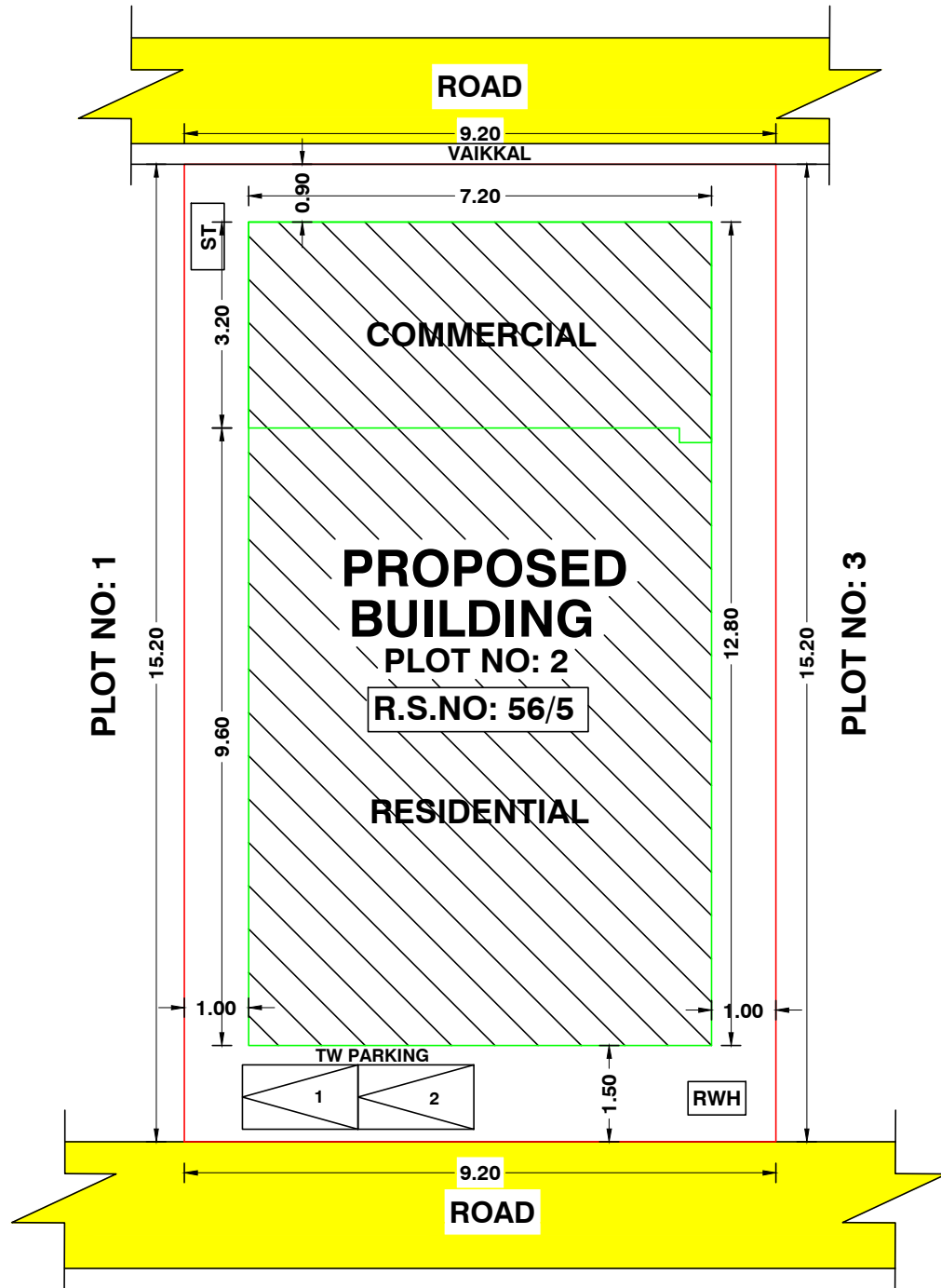
SITE PLAN
