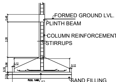
TYPICAL DETAIL OF COLUMN FOOTING
