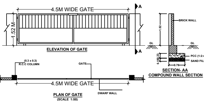
PLAN OF GATE (SCALE: 1:50)
