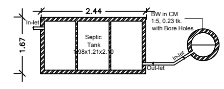
Plan - Septic tank & Soak pit
