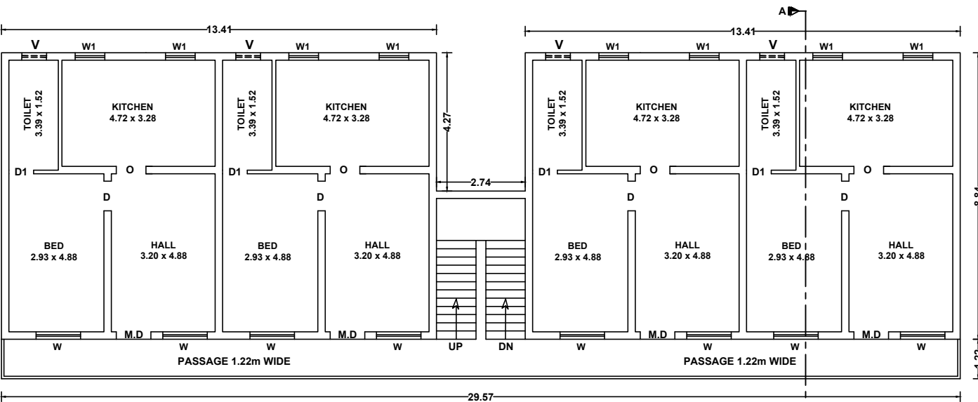
TYPICAL FLOOR PLAN FIRST & SECOND FLOOR
