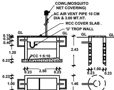
PLAN AND CROSS SECTION OF ST&SP.
