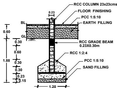
FOUNDATION DETAILS
