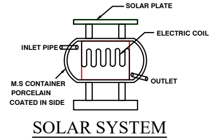
SOLAR SYSTEM
