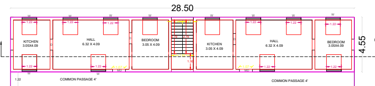
PRO.FIRST FLOOR PLAN
