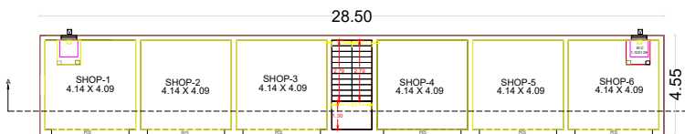
EXIS.GROUND FLOOR PLAN
