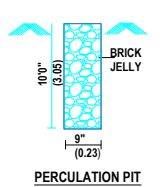
PERCOLATION PIT
