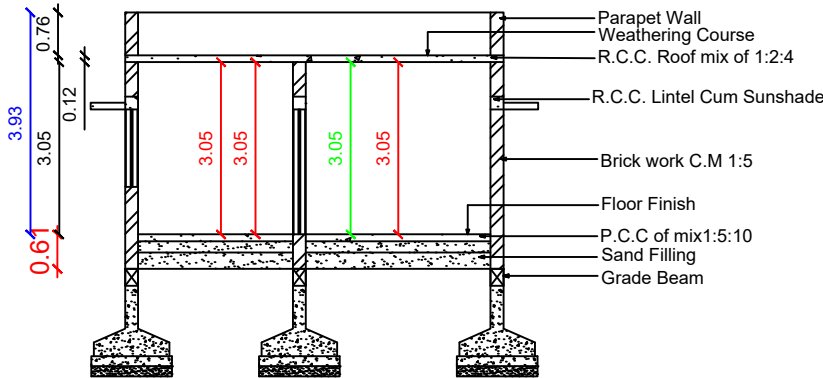
CROSS SECTION AB
