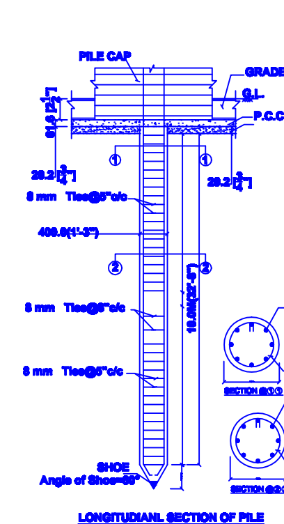
LONGITUDINAL SECTION OF PILE
