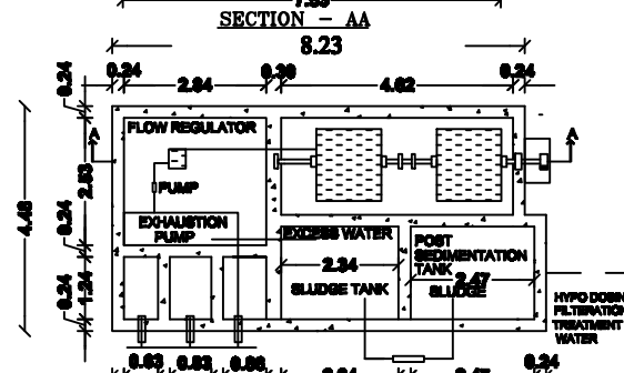
SEWAGE TREATMENT PLANT (S.T.P) WASTE WATER FILTRATION BY RECIRCULATION SYSTEM G.O.M.S.I NO.138 DT.11.10.22
