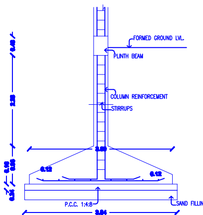
TYPICAL DETAIL OF COLUMN FOOTING
