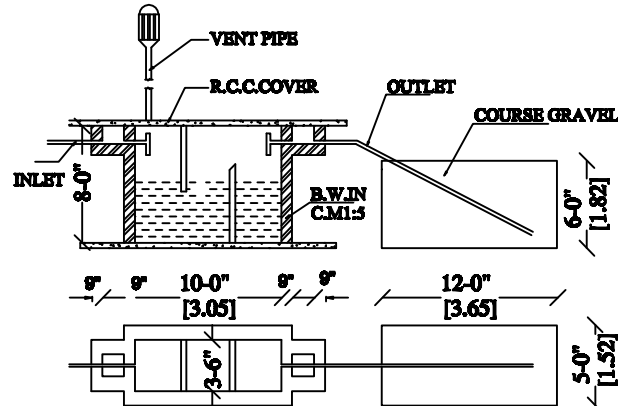
SEPTIC TANK & D-TRENCH DETAILS (NOT TO SCALE)
