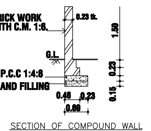
SECTION OF COMPOUND WALL
