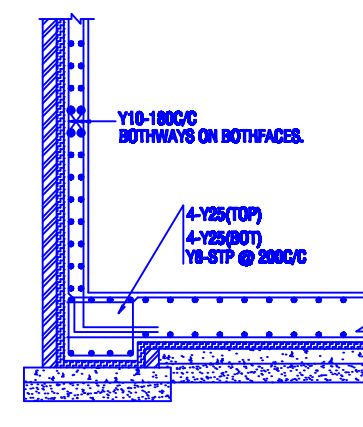
TYPICAL RAFT DETAIL
