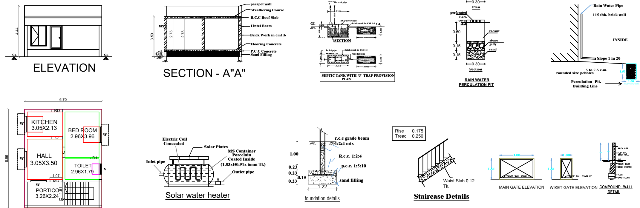
PRO.GROUND FLOOR PLAN
