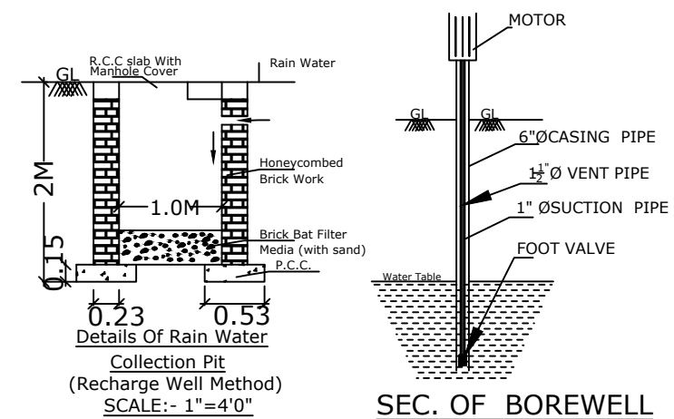
SEC. OF BOREWELL
