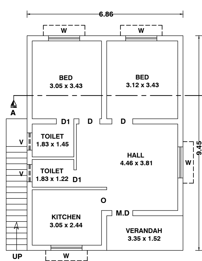
EXI. GROUND FLOOR PLAN
