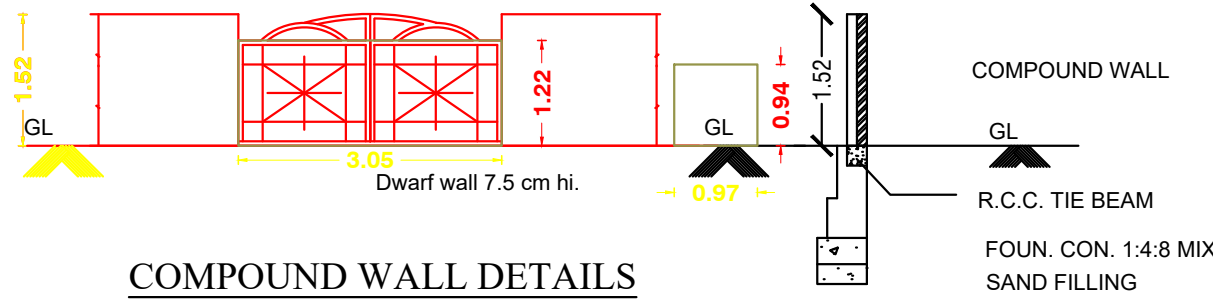
SECTION
