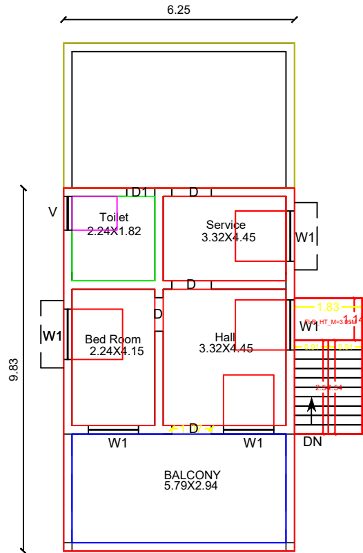
PRO..FIRST FLOOR
