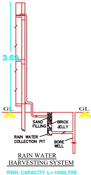
RAIN WATER HARVESTING SYSTEM RWHS_CAPACITY_L=1000LTRS
