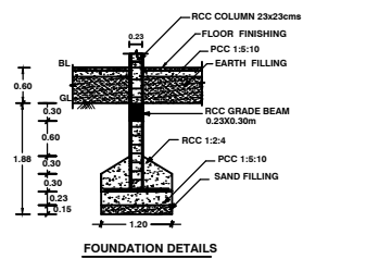
FOUNDATION DETAILS
