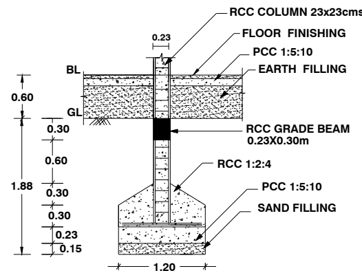
FOUNDATION DETAILS
