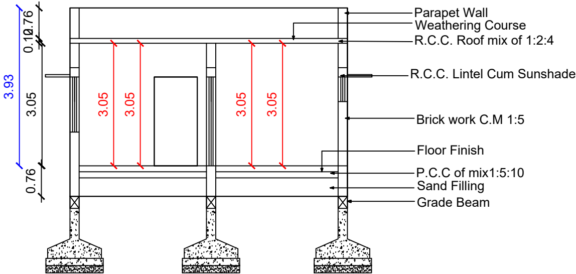
CROSS SECTION AB
