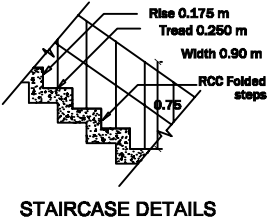
STAIRCASE DETAILS
