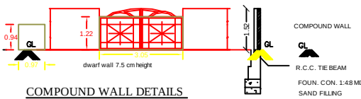
COMPOUND WALL DETAILS
