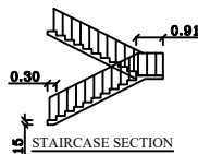
STAIRCASE SECTION
