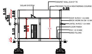
CROSS SECTION AB
