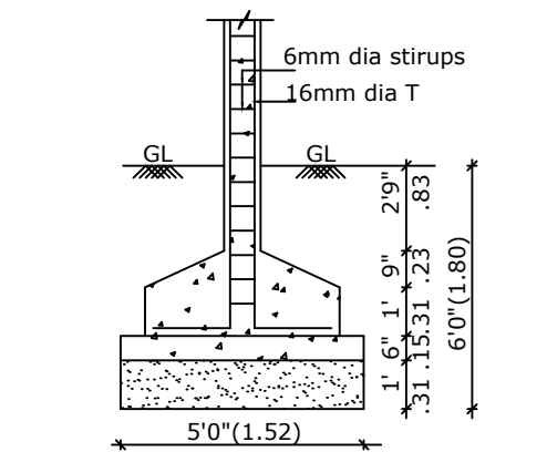
COLUMN FOUNDATION DETAIL
