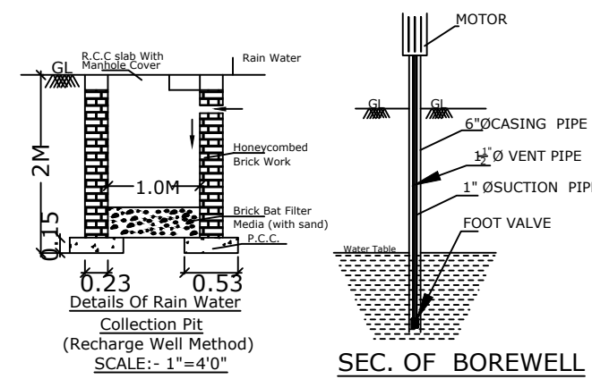
SEC. OF BOREWELL
