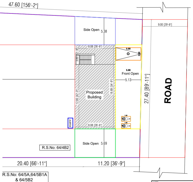
SITE PLAN
