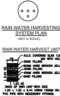
RAIN WATER HARVEST UNIT
