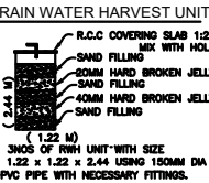
RAIN WATER HARVEST UNIT
