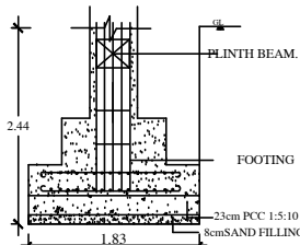
COLUMN FOUNDATION DETAILS NOT TO SCALE
