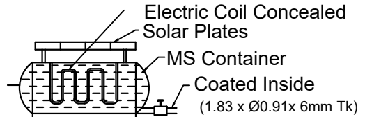
Solar water heater
