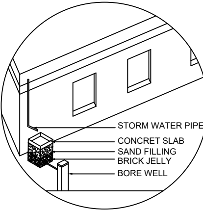
RAINWATER HARVESTING
