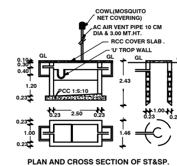
PLAN AND CROSS SECTION OF ST&SF
