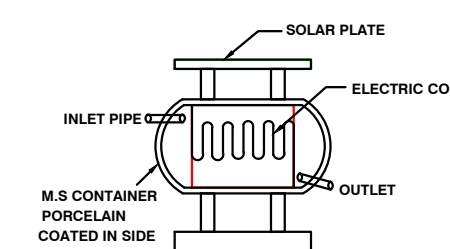
SOLAR SYSTEM
