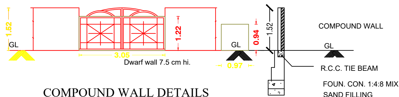
SECTION
