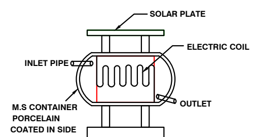
SOLAR SYSTEM
