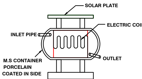
SOLAR SYSTEM
