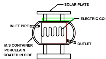
SOLAR SYSTEM
