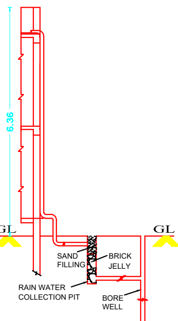
RAIN WATER HARVESTING SYSTEM RWH_CAPACITY_L=1000LTRS
