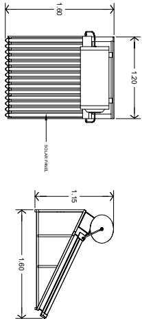
SOLAR WATER HEATER SYSTEM :- NOT TO SCALE
