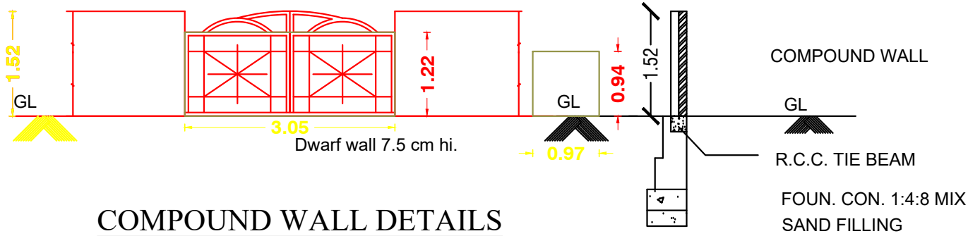
SECTION
