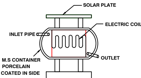
SOLAR SYSTEM
