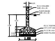
COLUMN FOUNDATION DETAILS
