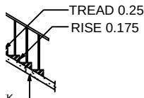
STAIR DETAILS
