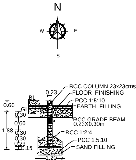
FOUNDATION DETAILS
