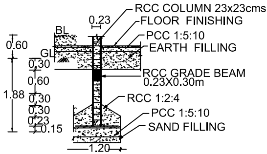
FOUNDATION DETAILS
