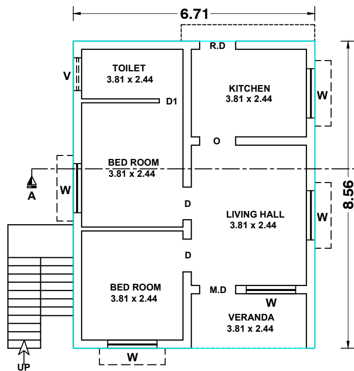
EXI. GROUND FLOOR PLAN
