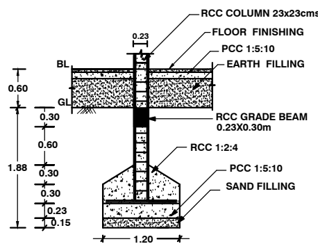
FOUNDATION DETAILS
