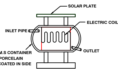
SOLAR SYSTEM
