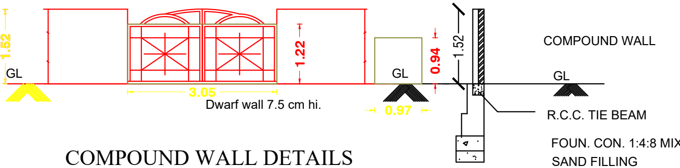
SECTION
